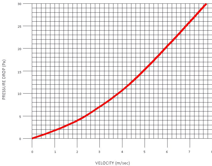
WAVEGUIDE VENT STATIC PRESSURE DROP
